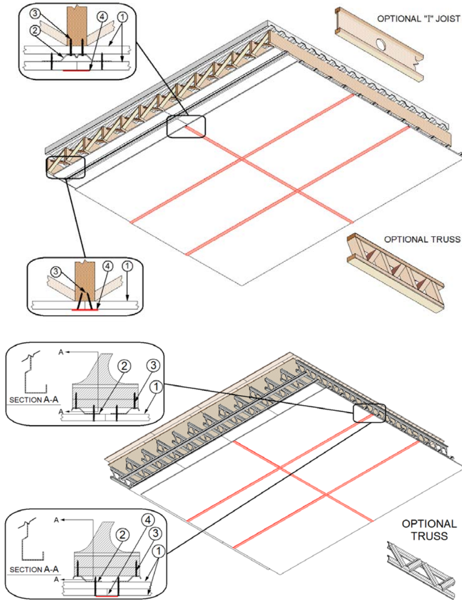
Figure 1 – Floor/Ceiling Assembly & Details
