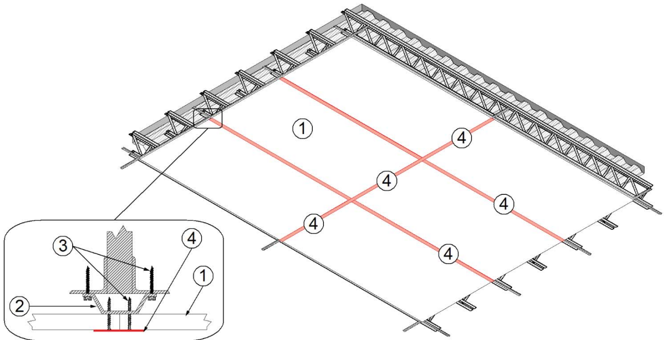
Figure 1 – Floor/Ceiling Assembly & Details
