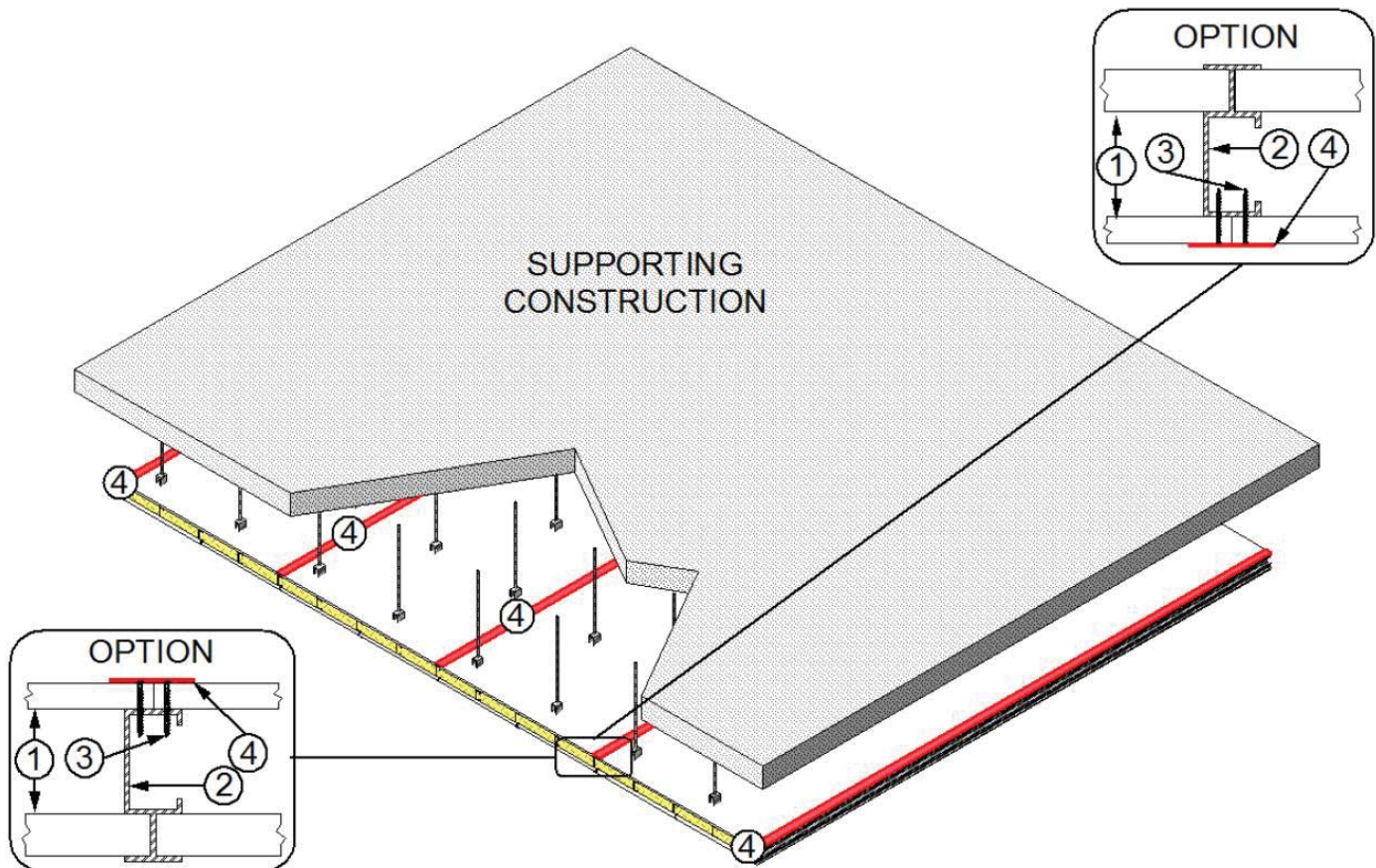
Figure 1 – Floor/Ceiling Assembly & Details
