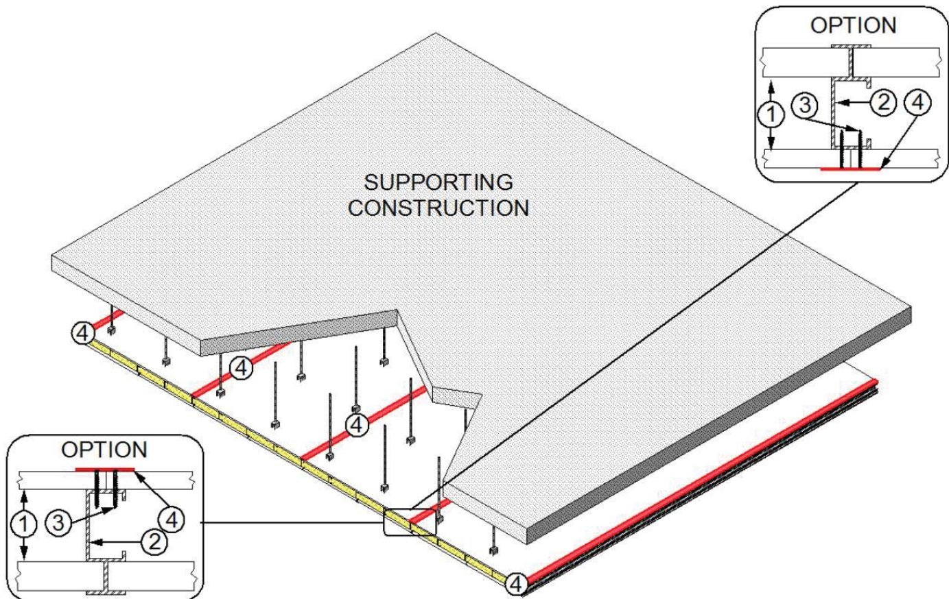
Figure 1 – Floor/Ceiling Assembly & Details
