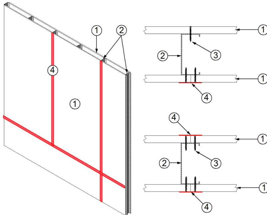
Figure 1 – Wall Assembly & Details
