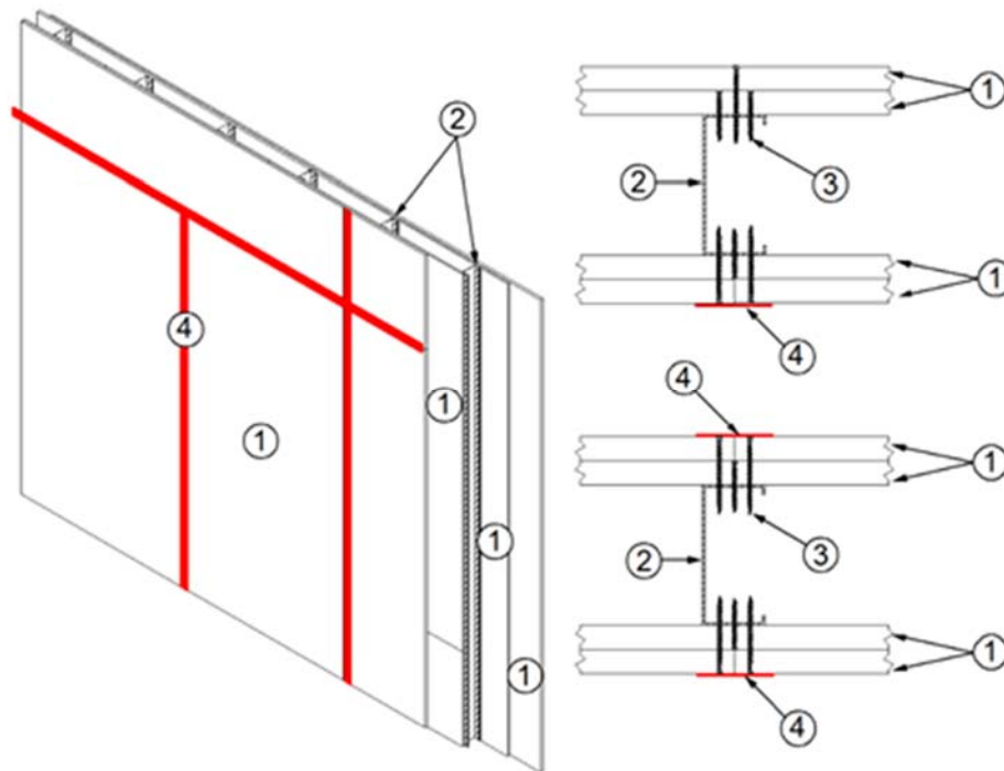
Figure 1 – Wall Assembly & Details
